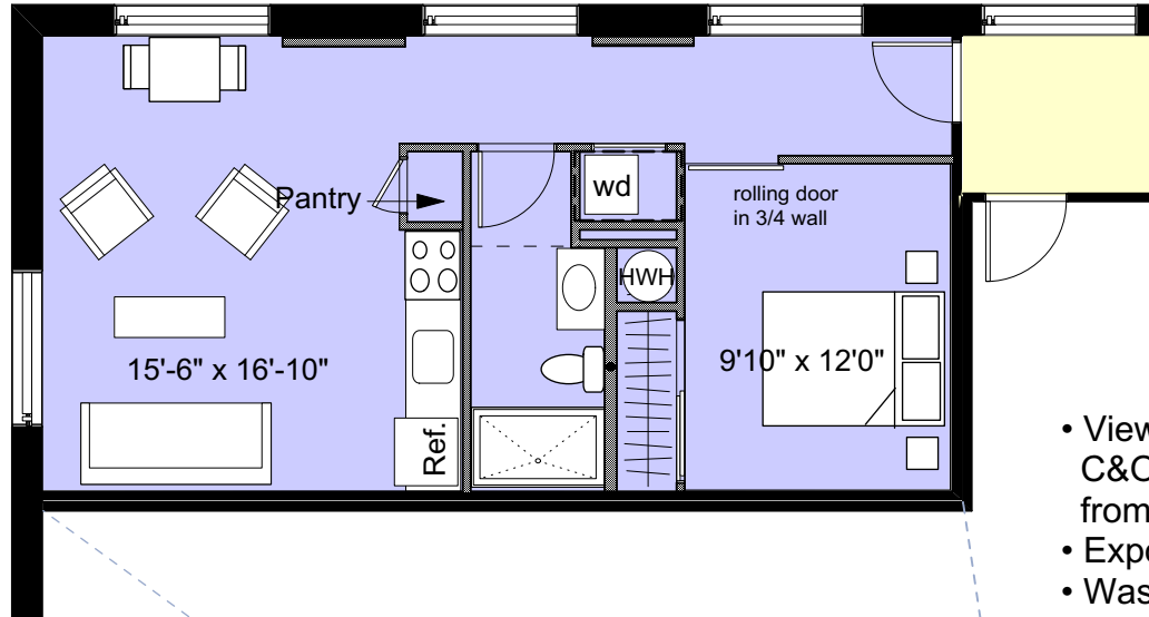
1 Unit 2A/3A/4A Plan Scale: 1/8" = 1'-0"
